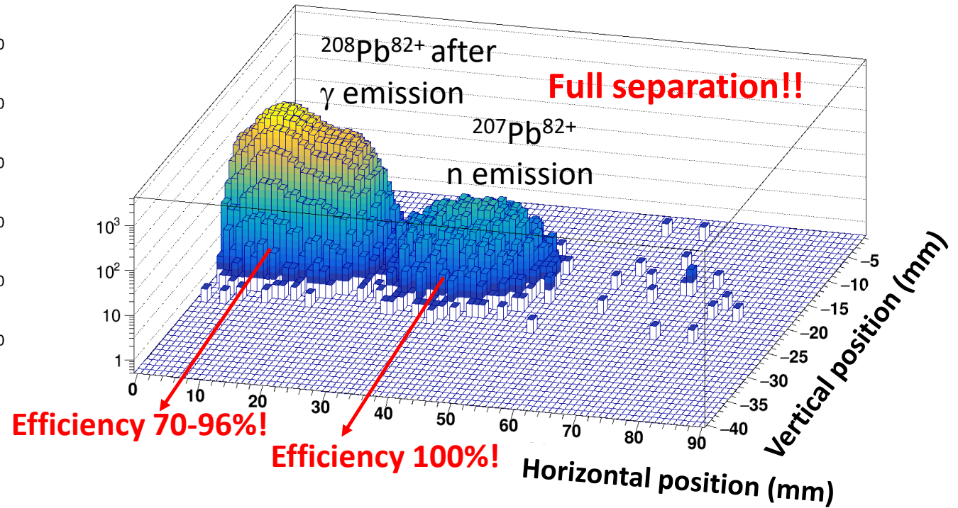
Position of detected beam residues in coincidence with protons
