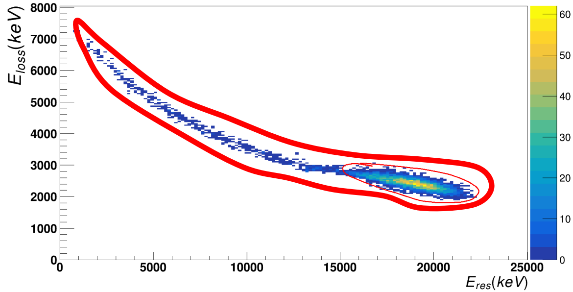
Detected protons
